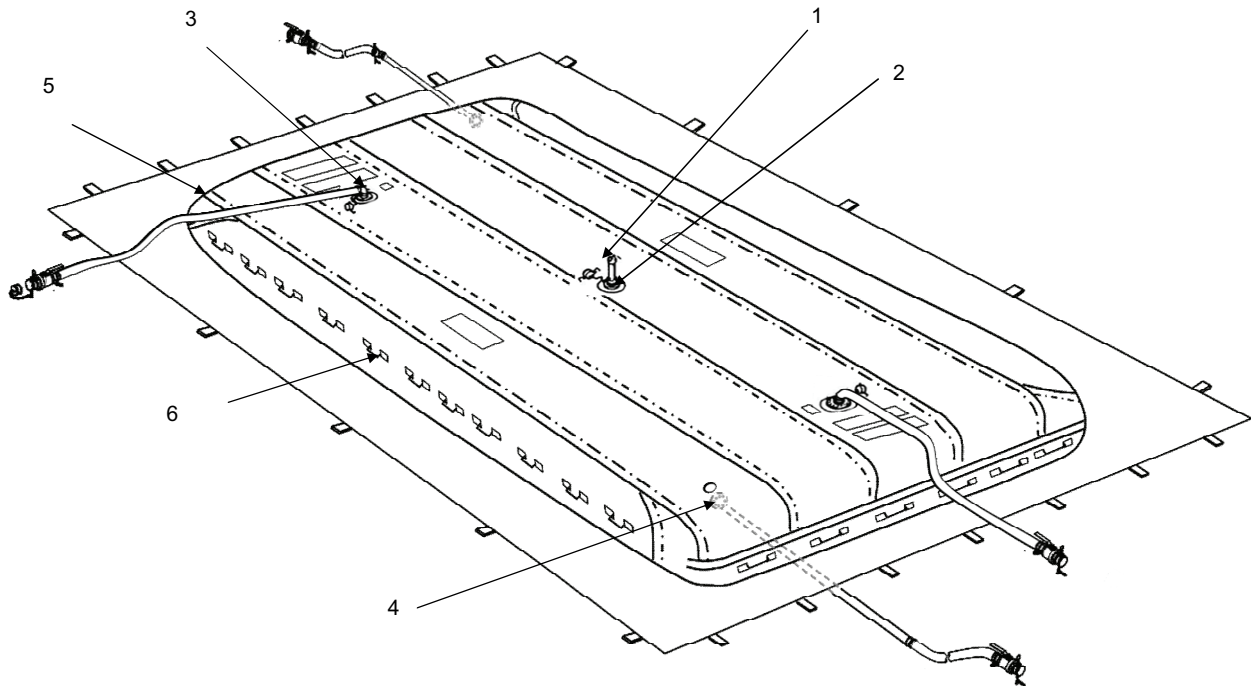
Figure 1. Tank Assembly.
