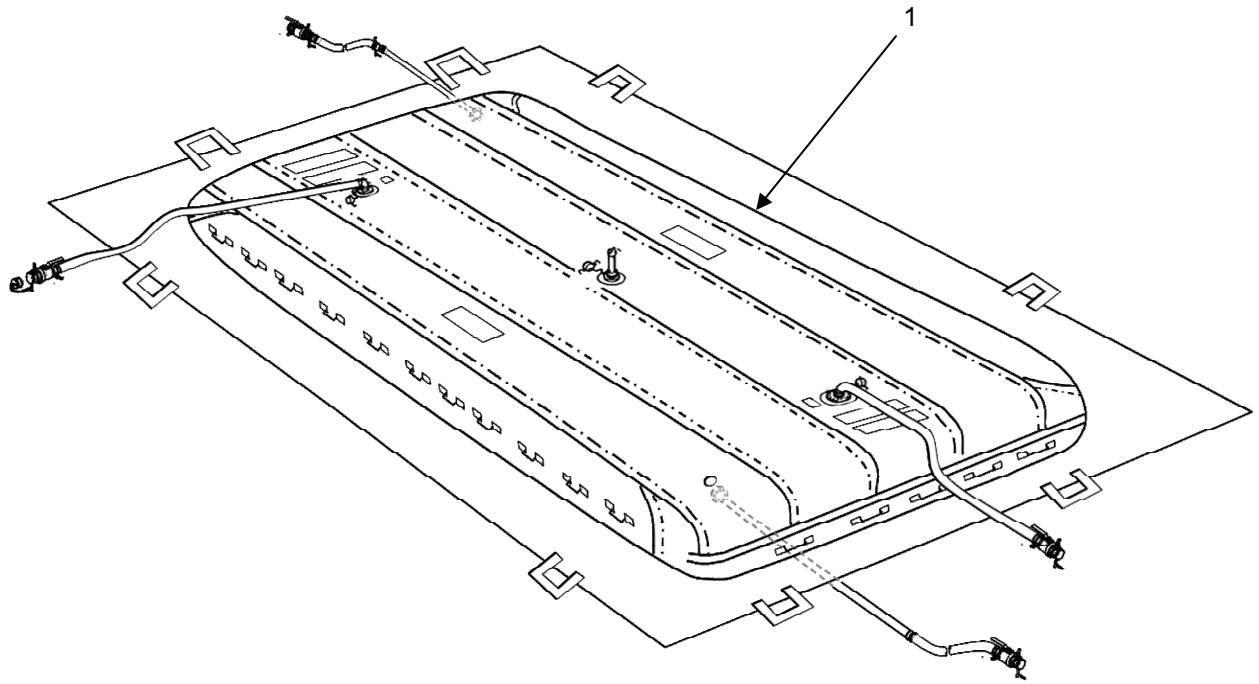
Figure 1. Tank Assembly.
