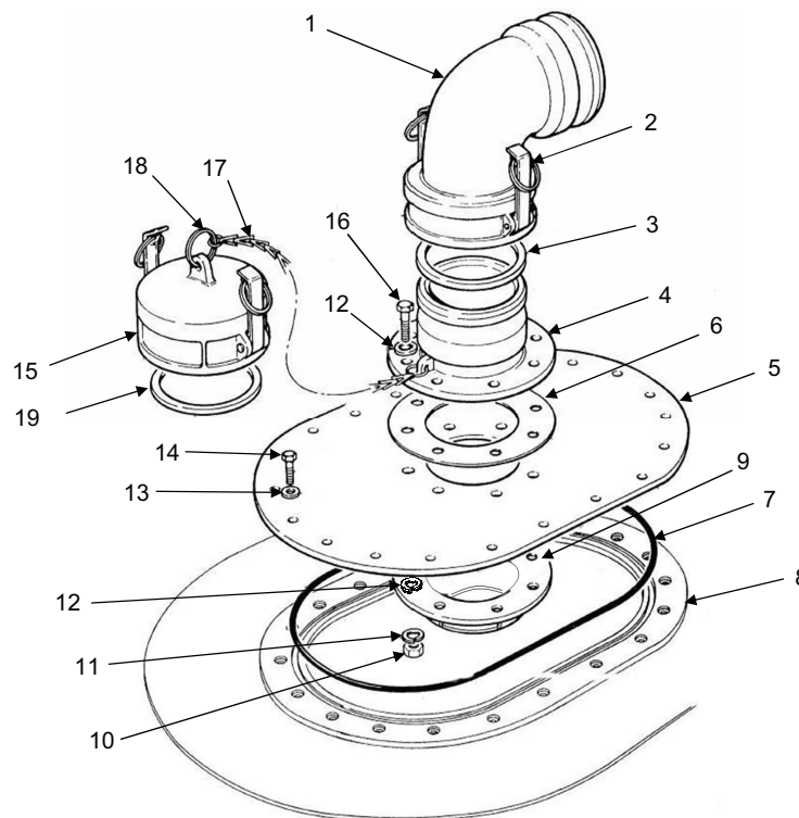
Figure 1. Filler/Discharge Assembly.
