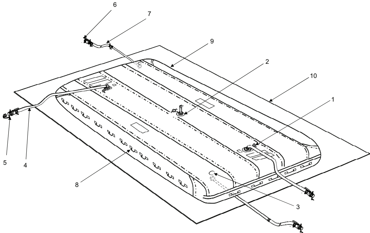
Figure 1. Tank Assembly.
