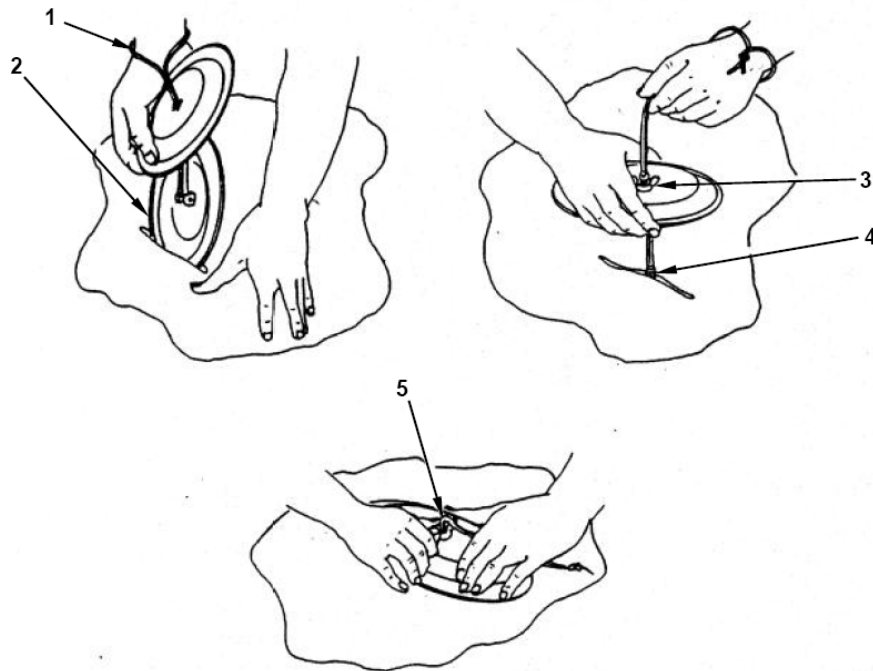
Figure 3. Installation of Mechanical Patches.
