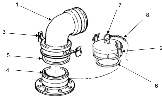
Figure 1. Filler/Discharge Assembly.
