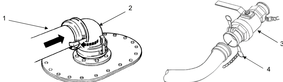
Figure 6. Filler/Discharge Hose Assembly.
